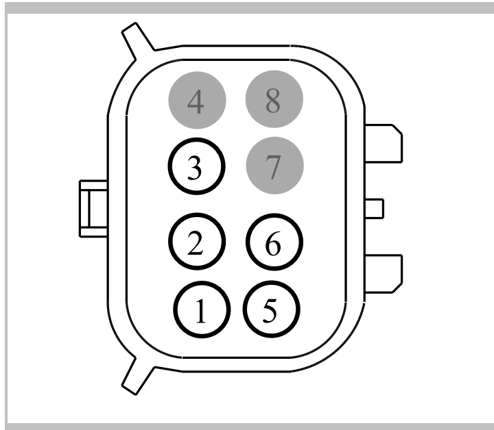
MALE Harness 12A581
