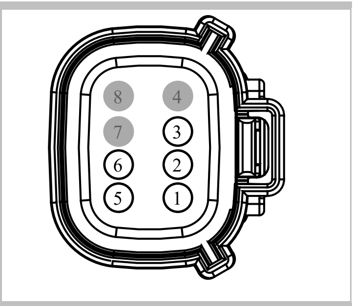
FEMALE Harness 3D097
